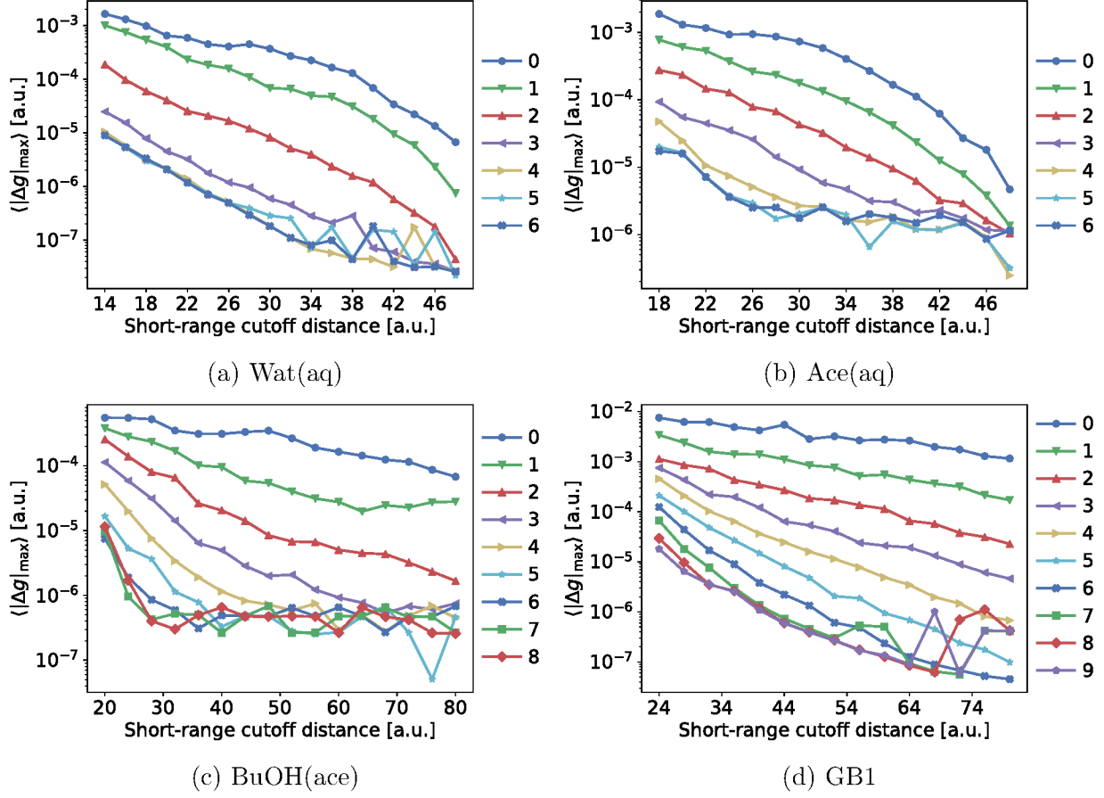
Figure 6: Convergence of the forces in (a) Wat(aq), (b) Ace(aq), (c) BuOH(ace), and (d) GB1 with respect to the short-range cutoff distance and the order of the multipole expansion used for the long-range coupling (which are indicated with different colors). The points show the mean of the maximum absolute error based on single-point calculations on ten snapshots using the full short-range coupling as reference. The cutoff distance is based on the fragment-based partitioning scheme in the case of Wat(aq), Ace(aq), and BuOH(ace), whereas for GB1 it is based on the atom-based partitioning.
