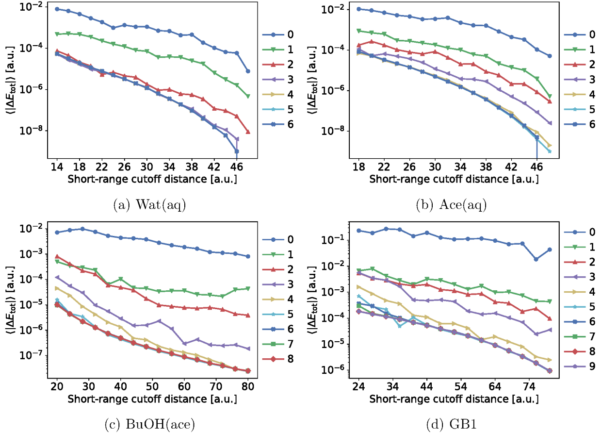
Figure 5: Convergence of the total energy of (a) Wat(aq), (b) Ace(aq), (c) BuOH(ace), and (d) GB1 with respect to the short-range cutoff distance and the order of the multipole expansion used for the long-range coupling (which are indicated with different colors). The points show the mean absolute error based on single-point calculations on ten snapshots using the full short-range coupling as reference. The cutoff distance is based on the fragment-based partitioning scheme in the case of Wat(aq), Ace(aq), and BuOH(ace), whereas for GB1 it is based on the atom-based partitioning.
